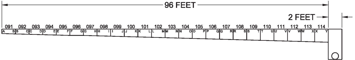
One Directional Trench Without Neutrals
