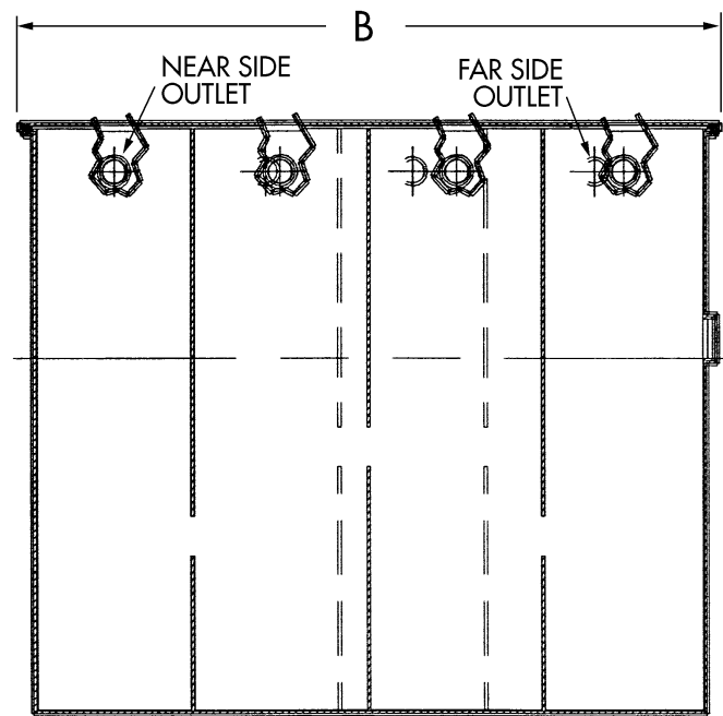
PLAN VIEW OF COMPARTMENT LAYOUT
