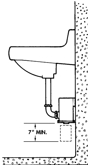
5750 Flush With Wall Installation
