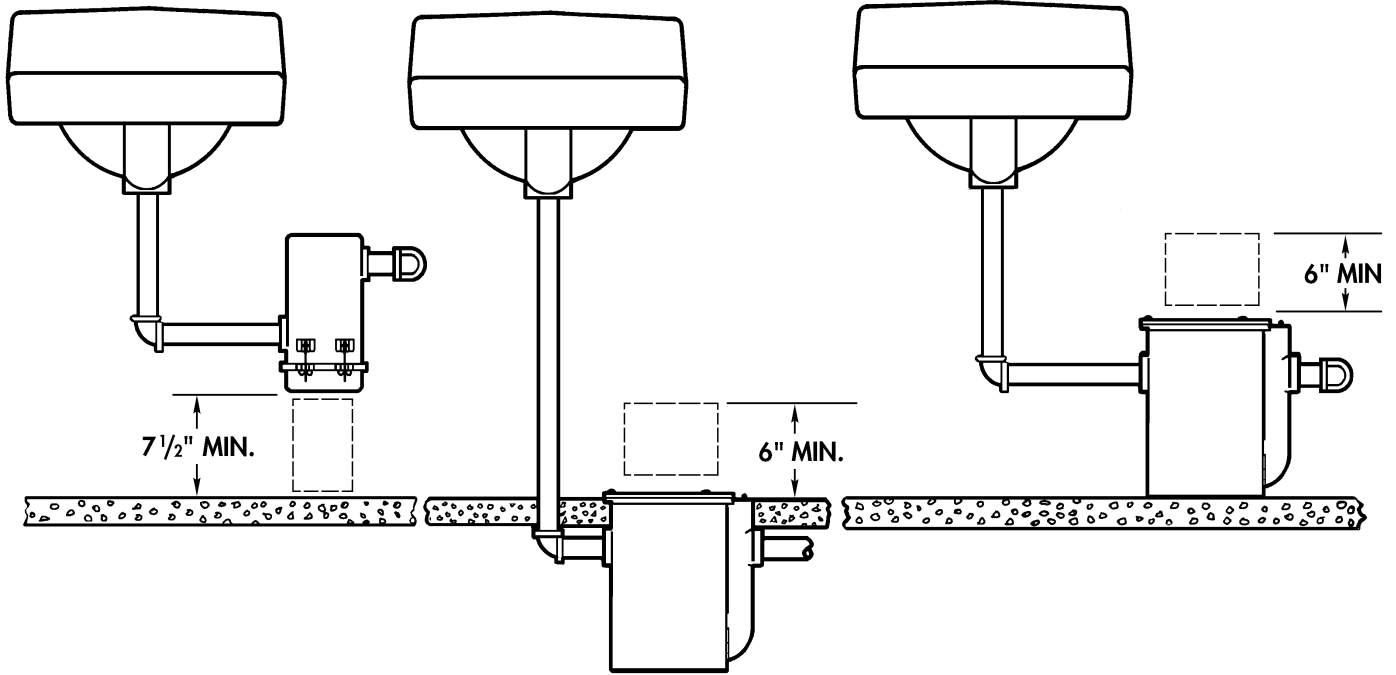
5730 Suspended Installation
