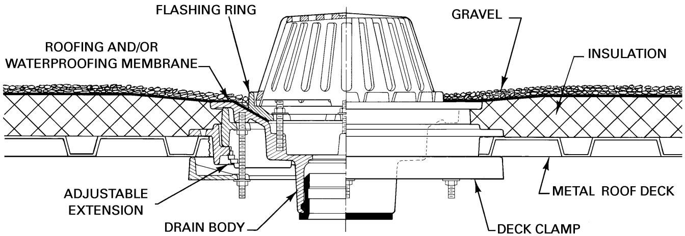
3000AE Roof Drain Installed In Insulated Metal Roof
