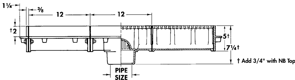
2950, 1 Ft, Outlet w/Two 2950, 1Ft, Extensions
